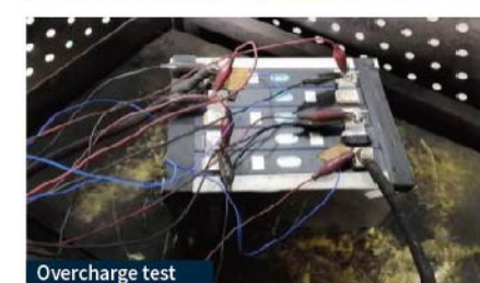
Overcharge test
